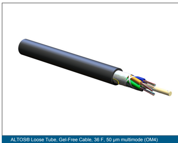
ALTOS® Loose Tube, Gel-Free Cable, 36 F, 50 µm multimode (OM4)
