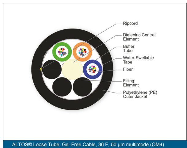
ALTOS® Loose Tube, Gel-Free Cable, 36 F, 50 µm multimode (OM4)
